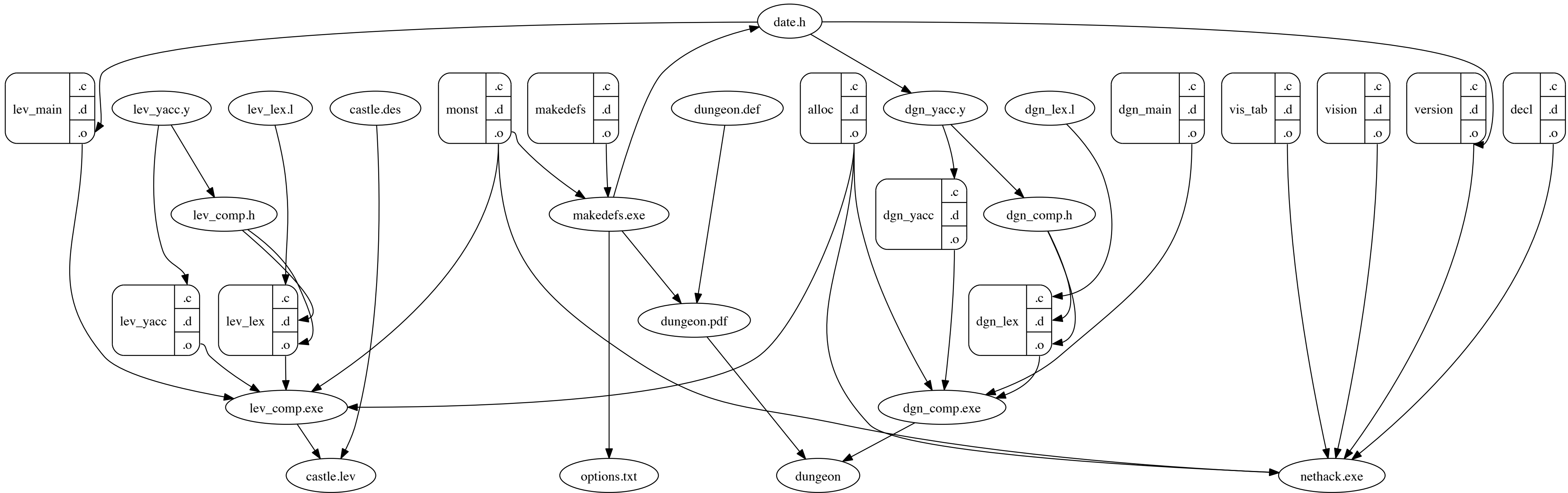
Abbreviated Nethack Build Dependencies
